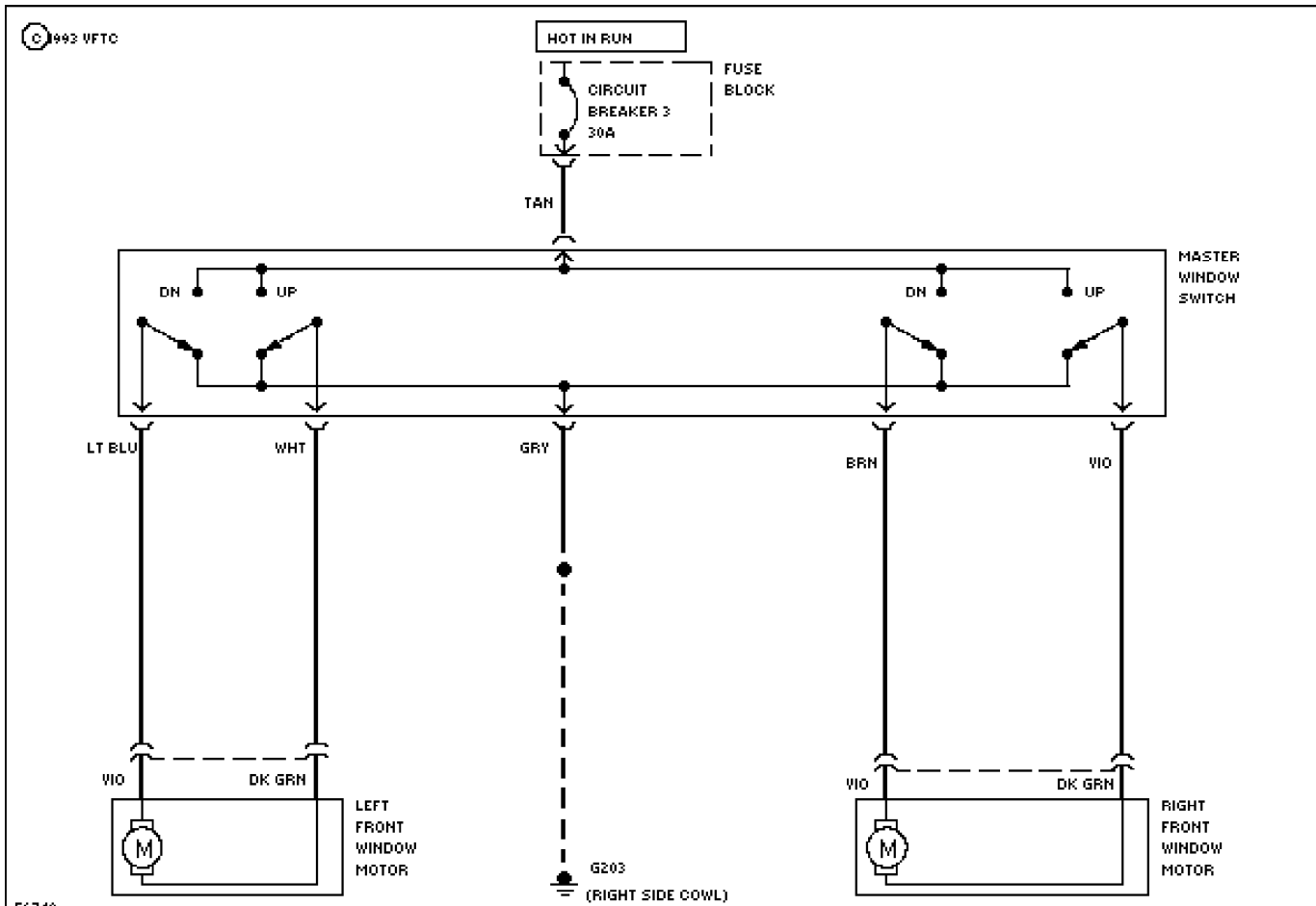
Power Windows Circuit, 2 Door Hardtop
