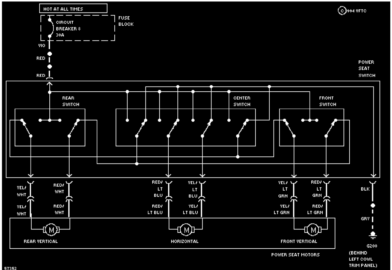
Left Seat Circuit
