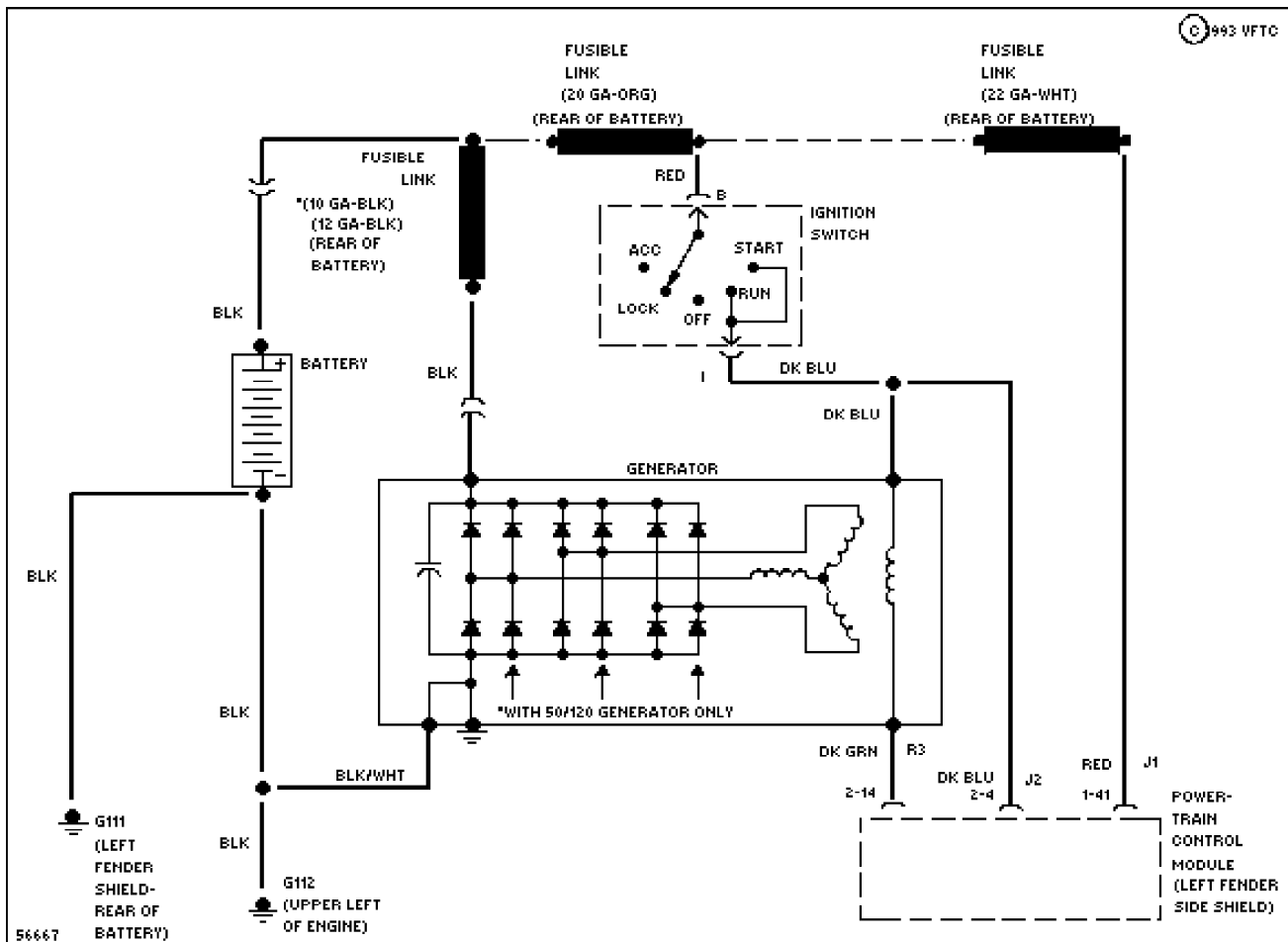
Charging Circuit
