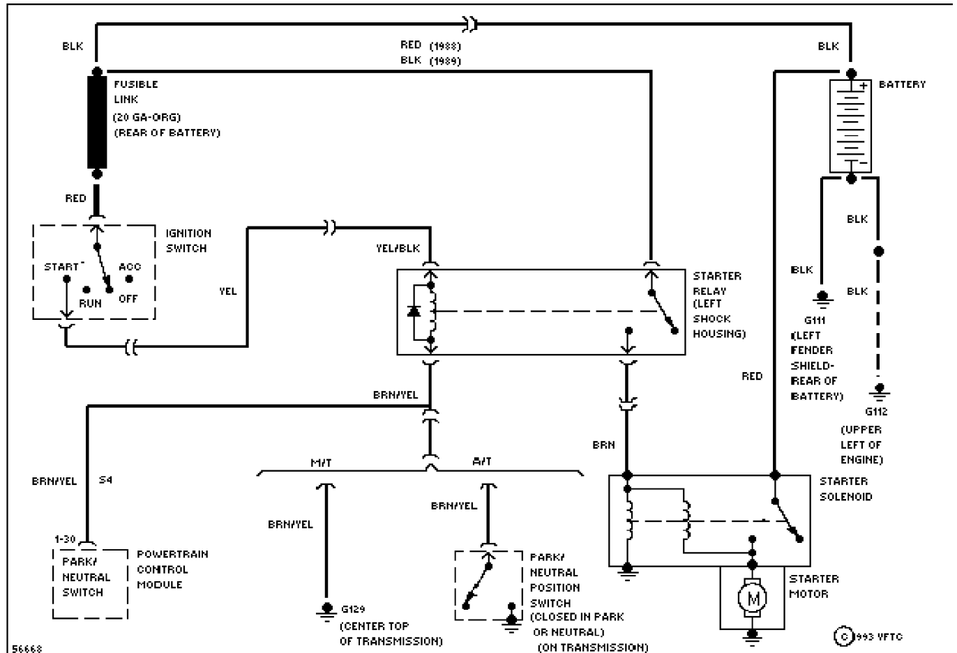
Starting Circuit
